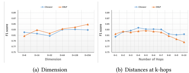
Figure 2: Parameter analysis on D and K -hops
